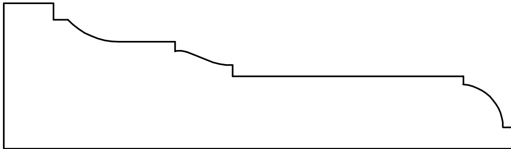
F-2109 1.500" x 5.250" New Era
