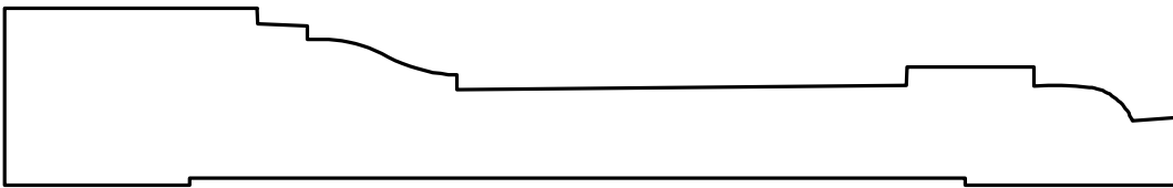
F-2927A 0.8316" x 5.5377" Balt. Design & Build
