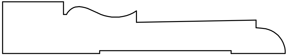
F-2675 .855" x 4.692" Pyramid Construction
