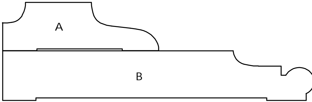
F-2770 A- 0.832" x 2.678" B- 0.855" x 5.342" Bauer
