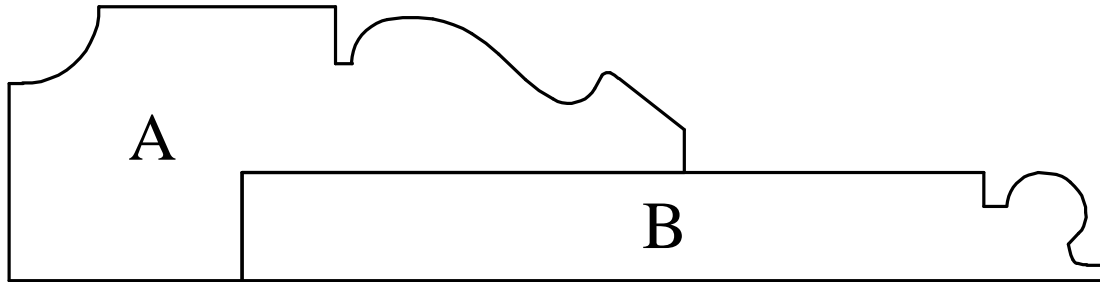
F-2825 A - 1.4257" x 3.5176" B - .5625" x 4.500" Lidco
