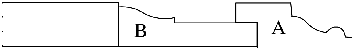
F-8137 A- 0.796" x 2.048" B- 0.701" x 2.398" Red Door
