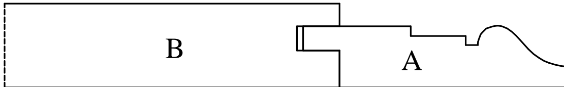
F-8055 A-0.638" x 2.717" B-0.866" x 6.125" Roy Cox
