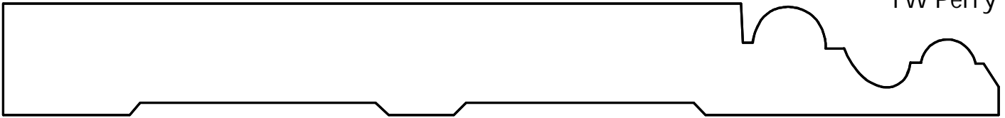
F-8212 .8174" x 7.2972" TW Perry
