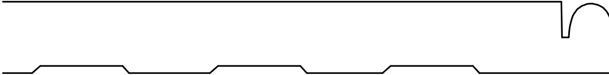
F-8235 0.7353" x up to 9" Cabinet Max
