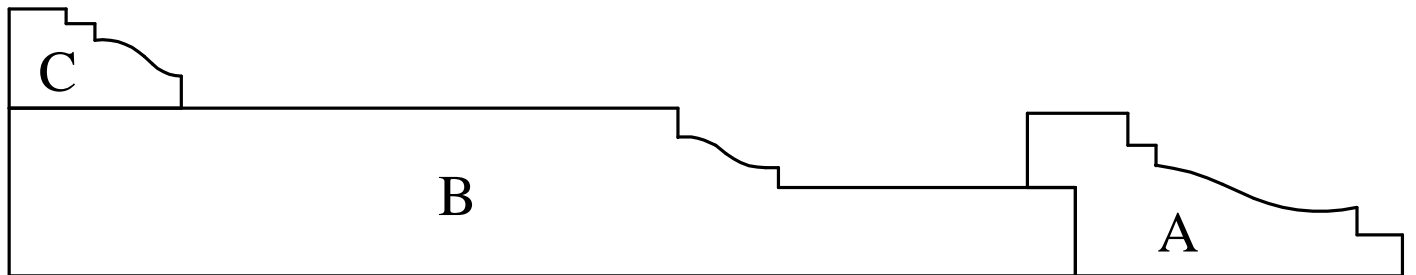
F-8076 A-0.847" x 1.957" B-0.875" x 5.557" C-0.516" x 0.897" McClees
