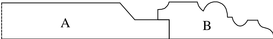
F-8091 A- 0.802" x up to 9" B- 0.825" x 2.546" Norris
